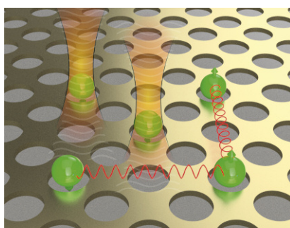
Figure 1: Atoms trapped in grid simulating the correlations in a molecule.
