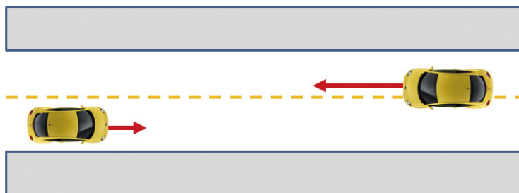
Figure 2: Probability and location of possible collision between two vehicles (interference between two quantum walkers).
