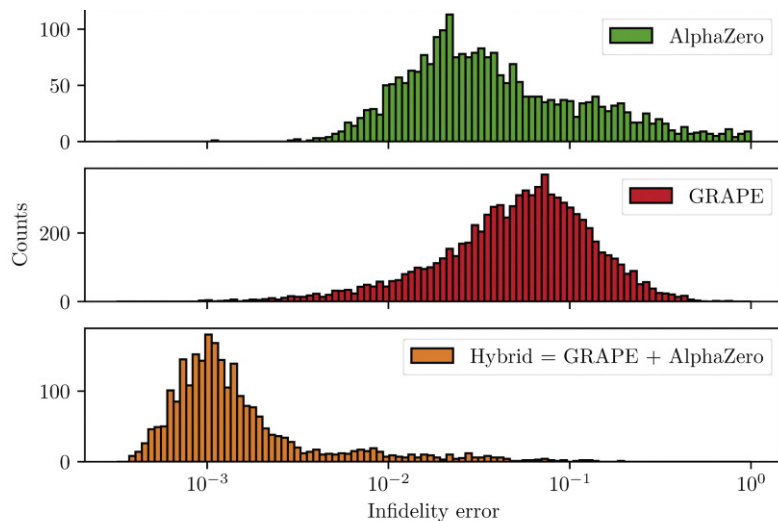
Figure 1: The infidelity error (lower is better) for making a quantum computational gate that could potentially be used in a quantum computer. The figures show the results of three different methods: A deep learning algorithm, AlphaZero, a local gradient-based optimisation algorithm, GRAPE, and a hybrid algorithm that combines the two. Results are taken from [2].
