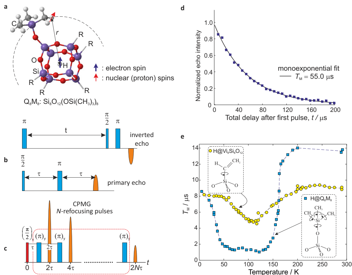
Figure 1: a) Encapsulated atomic hydrogen in a POSS cage with R=\text{OSi}(\text{CH}_3)_3 , \text{H}@Q_8M_8 . Only one of the eight groups R is displayed. b) Pulse sequences for measuring T_1 (upper) and T_M (lower). c) Carr-Purcell-Meiboom-Gill (CPMG) pulse train. d) Dynamical decoupling with the CPMG microwave pulse sequence showing the electron spin echo decay measured at T=200 \text{ K} with N=30 refocusing \pi -pulses as a function of the time delay between the first \pi/2 -pulse and the occurring echoes, t=2\tau, 4\tau, \dots, 2N\tau . e) Temperature dependence of phase memory times T_M for two \text{H}@POSS species with different organic substituents, R .
