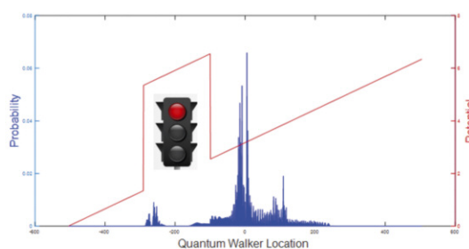
Figure 1: (a) vehicle accelerating to the right. (b) A vehicle decelerating in the presence of a red traffic light modelled as a potential barrier.
