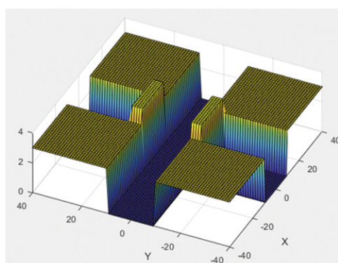
Figure 3: Urban areas are modeled by constant potential barriers (sidewalks and buildings) and time-varying potential barriers (traffic lights).
