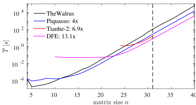
Figure 1: Benchmark comparison of individual implementations to calculate the permanent of an n \times n unitary matrix. For better illustration, the discrete points corresponding to the individual matrices are connected by solid lines. The numbers associated with the individual implementations describe the speedup compared to TheWalrus package at matrix size indicated by the vertical dashed line.
