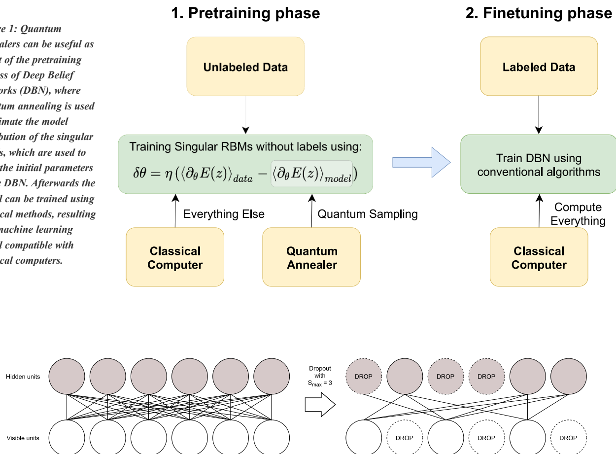
Figure 2: We use a variant of the Unit Dropout method, where S_{max} units are “dropped” stochastically for the duration of a single batch. This allows for larger layer sizes to be embedded to quantum annealing devices than would be conventionally possible.
