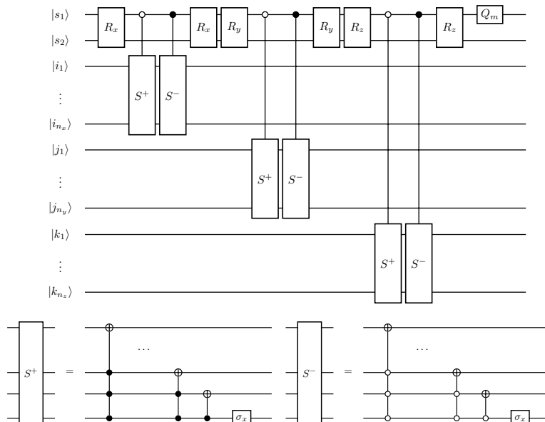
Figure 1: Quantum circuit for one time step of the free Dirac equation algorithm. The shift operator are denoted by S and the rotation operator by R . Adapted from Ref. [1].
