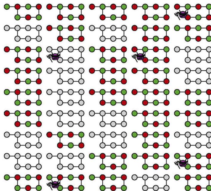
Figure 1: Each connected graph represents a given measurement-based pattern that is executed by the server, where each node in the graph represents a qubit. When a grey pattern is executed, it corresponds to the computation delegated by the client, while green and red ones represent delegated test rounds. Because the delegation is executed blindly, the malicious server (purple demon) does not know where to attack the computation, it inevitably gets detected by some test rounds. The advantage of the scheme is to ensure that each executed pattern has the same requirement as the computation itself while giving cryptographic guarantees with exponentially low correctness and soundness errors at the expense of a polynomial number of delegated rounds.
