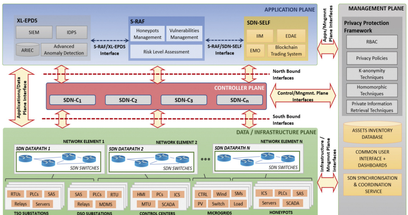
SDN-microSENSE architecture with functional blocks and interfaces.
