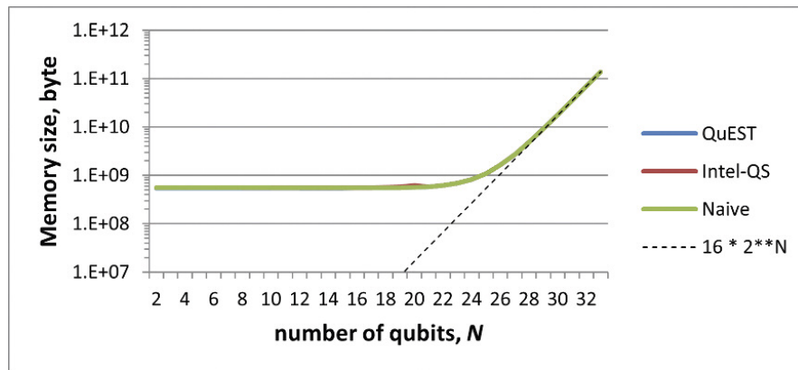
Figure 1: Total memory size needed to emulate a random Hadamard-cNOT circuit on the ENDEAVOR cluster, as a function of N .
